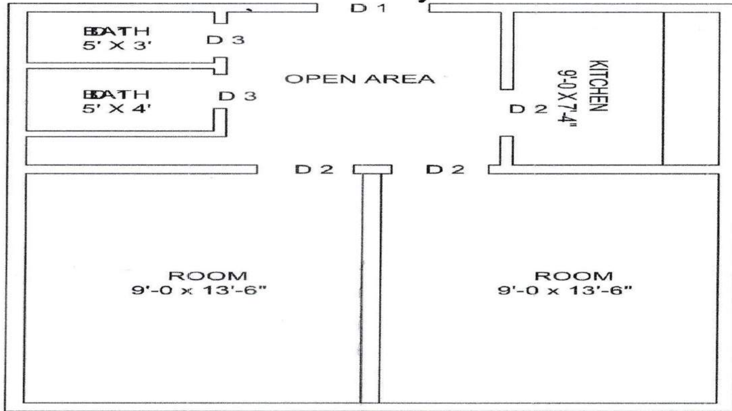
H-TYPE PLAN
