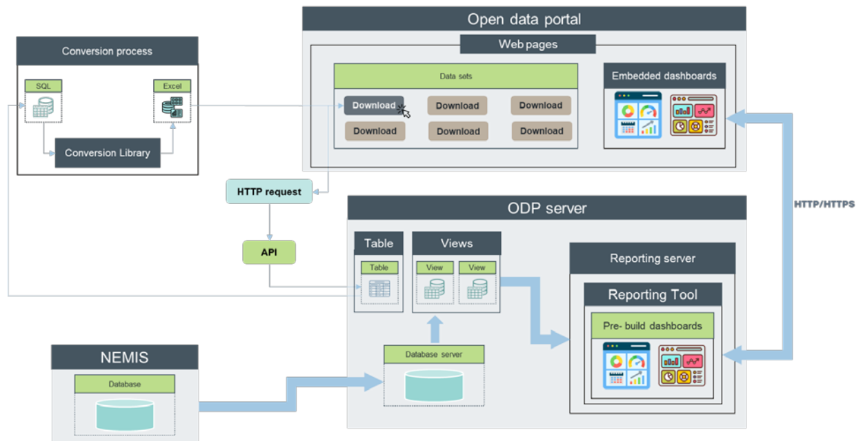
Architecture of the NODP Proposed under Design Document for National Open Data Portal
