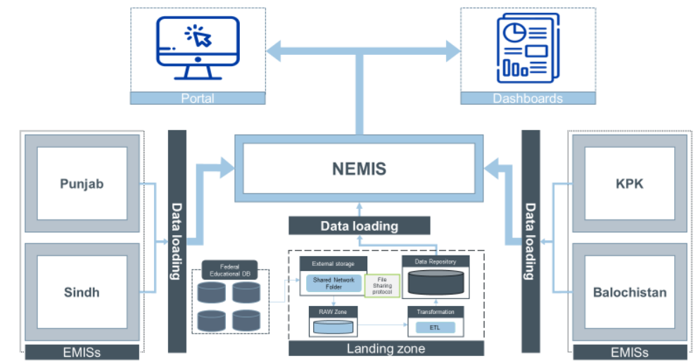
NEMIS Architecture (Vertical Integration) [Ref: Design & Architecture Horizontal & Vertical Integration]
