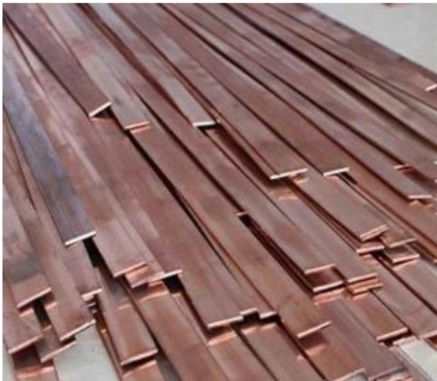
Picture-6 Copper Bar length \geq 1.5 meter (width 5cm, thickness 3mm)
