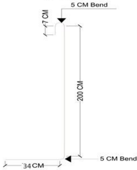
(SHAPE-05) Cut Length of Vertical Bar (COLUMN)
