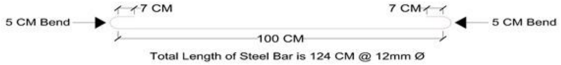
(SHAPE-04) Cut Length of Main & Distribution Bar (FOOTING)
