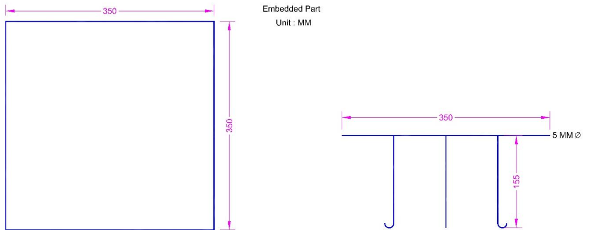
i) Profile View of the Embedded Part for Observation Room Fixing
