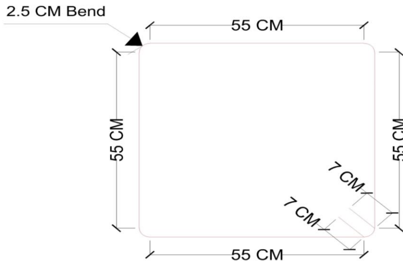
(SHAPE-02) Cut Length of Strips (WALL)
